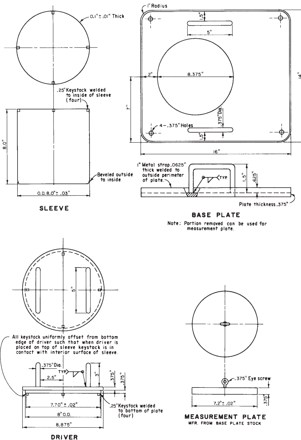
FIG. 1 Density Sleeve Apparatus
