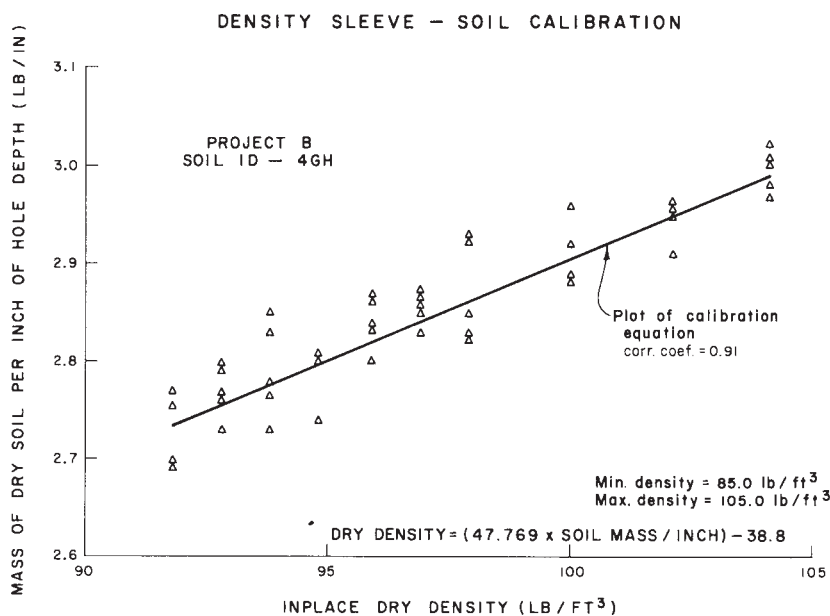
FIG. A1.3 Plot of Calibration Equation
