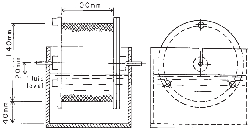
FIG. 1 Critical Dimensions of Slake Durability Equ Devipmce Showing Critical Dimensions
