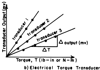
FIG. 5 Determination of Calibration Factors for Vane Torque Units
