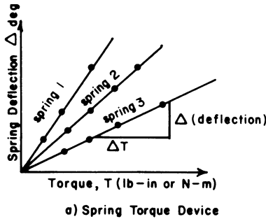
a) Spring Torque Device
