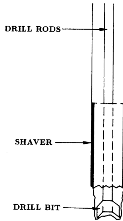
FIG. 7 Preparing the Test Cavity by the Pilot Hole Drilling and Simultaneous Shaving Technique
