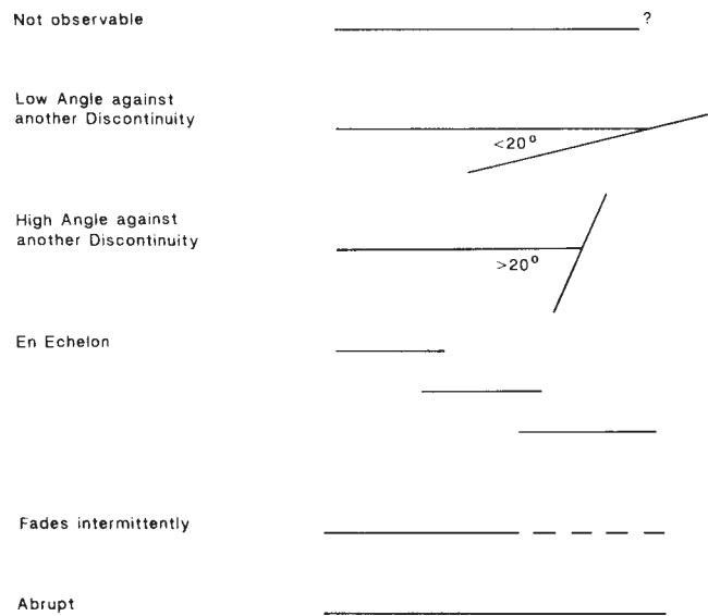
FIG. 3 Discontinuity Termination Types
