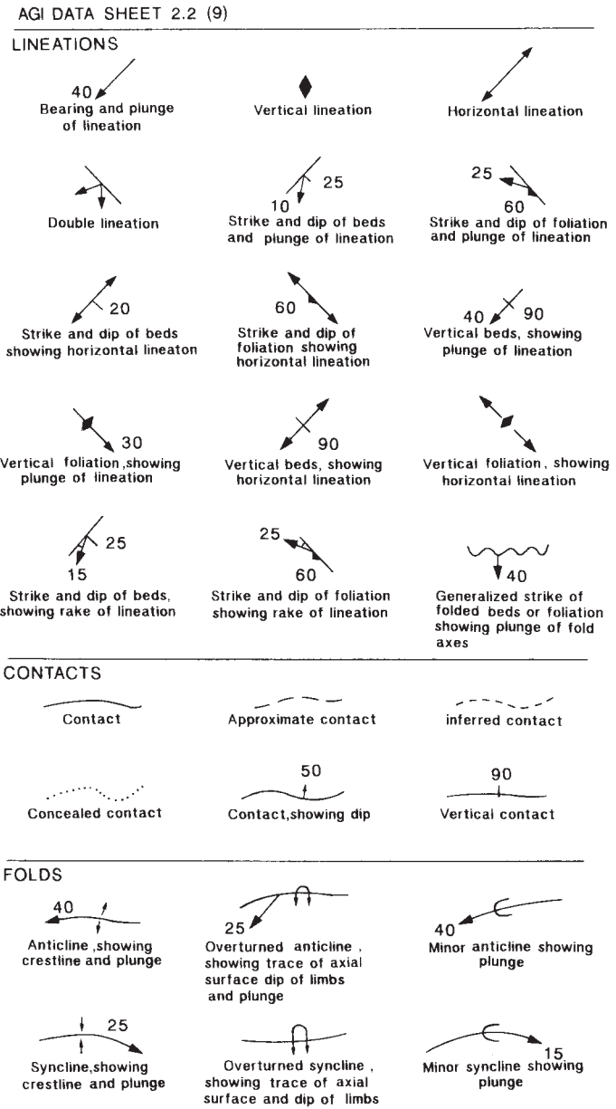
FIG. 1 Data Sheets of Mapping Symbols (9)
