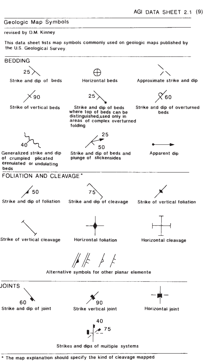
FIG. 1 Data Sheets of Mapping Symbols (9)
