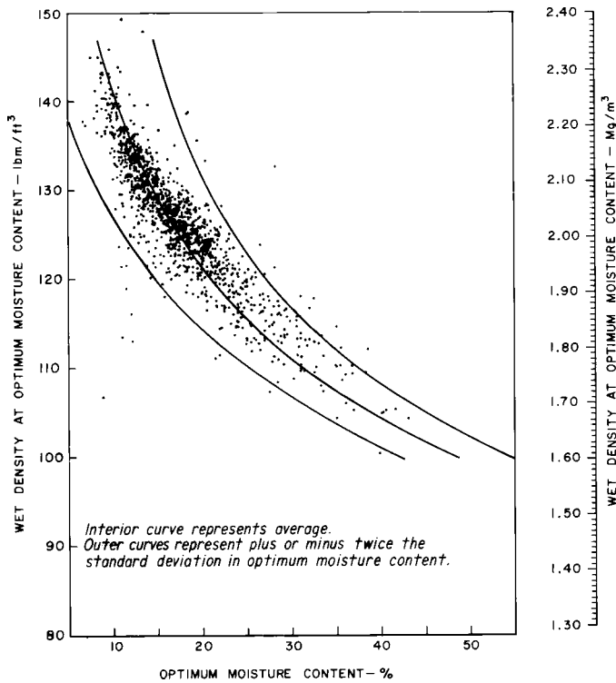
FIG. X2.1 Wet Density Versus Optimum Moisture Content
