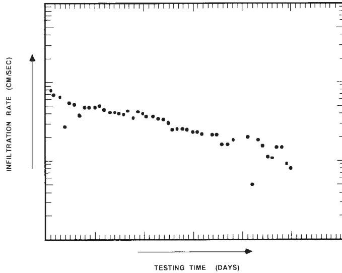
FIG. 5 Infiltration Rate Versus Time On A Semi-log Plot
