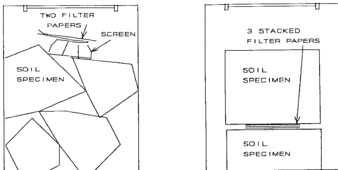
A. Total Suction B. Matrix Suction FIG. 2 Setup for Equilibrating Suction in Large Container
