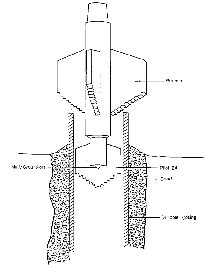
FIG. 3 Over Drilling by Mud Rotary Procedure
