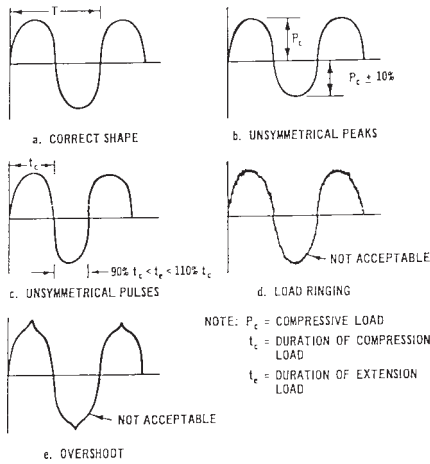
FIG. 3 Examples of Acceptable and Unacceptable Sinusoidal Loading Wave Forms for Cyclic Triaxial Strength Tests
