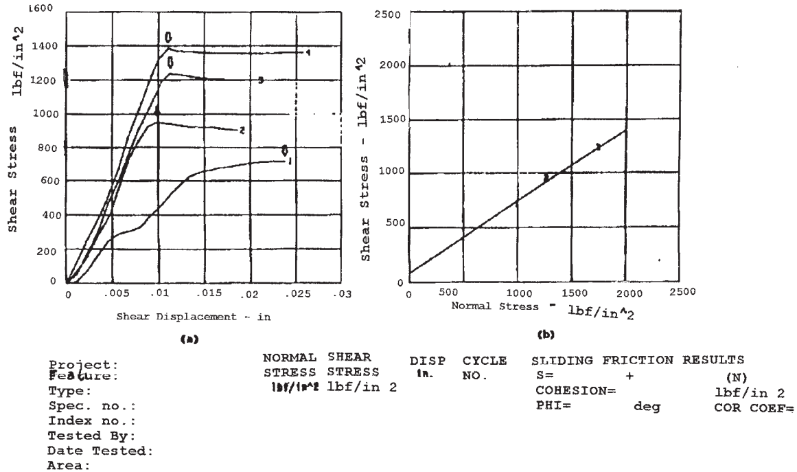
FIG. 8 Typical Presentation Sliding Friction Test Results: (a) Shear Stress and Shear Displacement and (b) Shear Strength and Normal Stress
