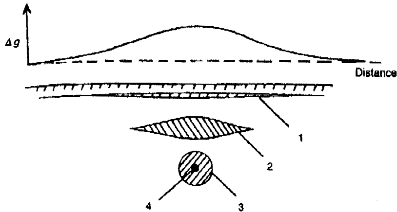
FIG. 4 Ambiguity in Gravity Interpretation (from Sharma (14))
