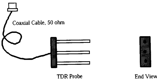
FIG. 4 Typical 3-Rod TDR Probe Configuration
