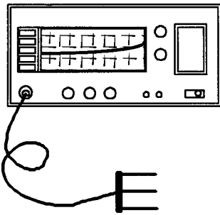
FIG. 2 Basic TDR System
