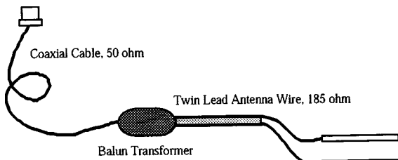
FIG. 5 Typical 2-Rod TDR Probe With Balun Transformer
