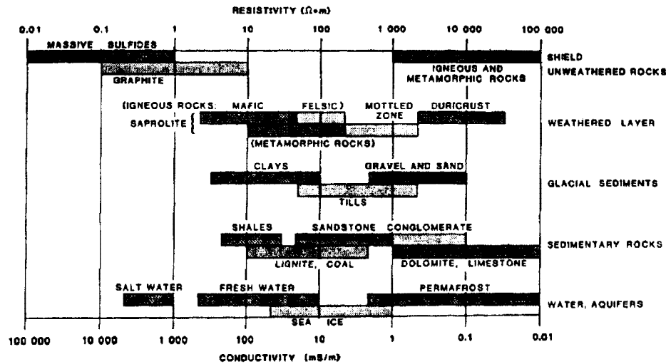
FIG. 6 Earth Material Conductivity Ranges (Sheriff, 1991)
