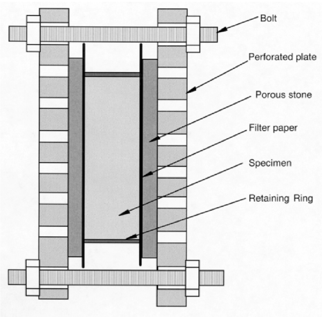
FIG. 11 Assembly Used to Contain Specimens When Saturating in a Saturation Chamber
