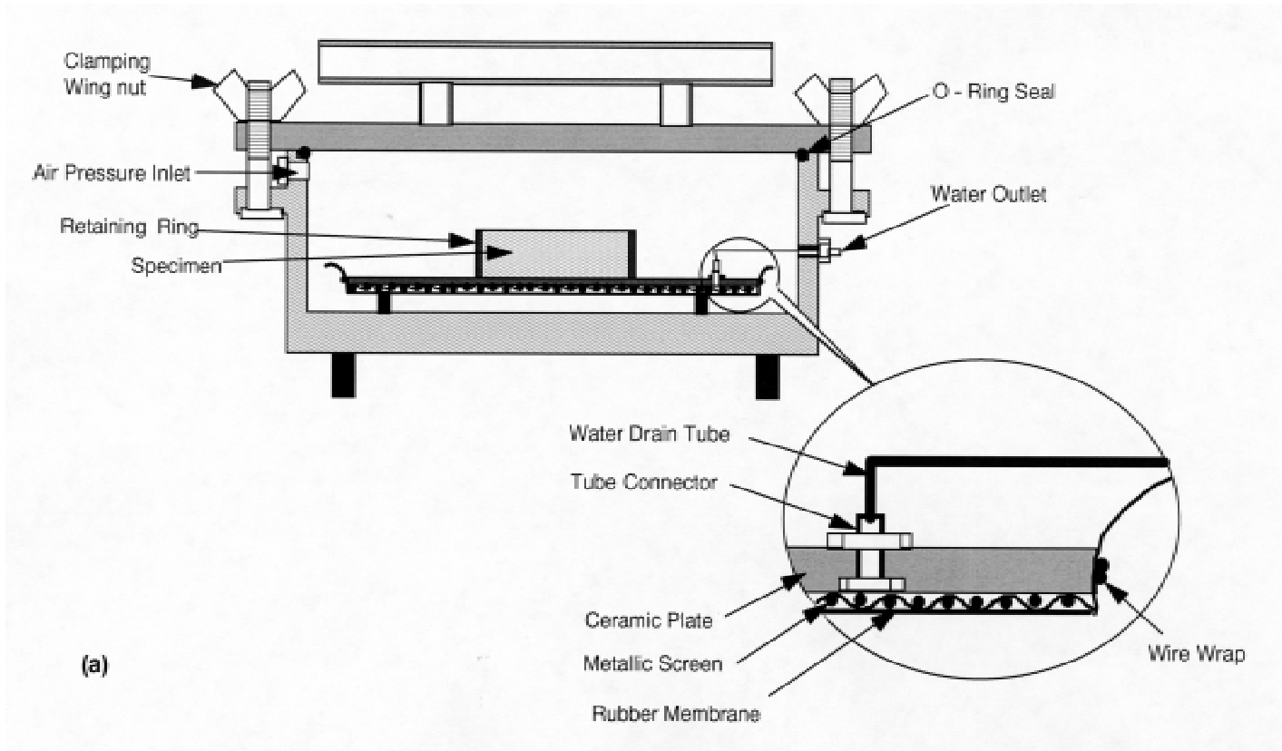
Schematic of pressure chambers with ceramic porous plates: (a) conventional chamber for single or multiple specimens and (b) chamber for single specimen
