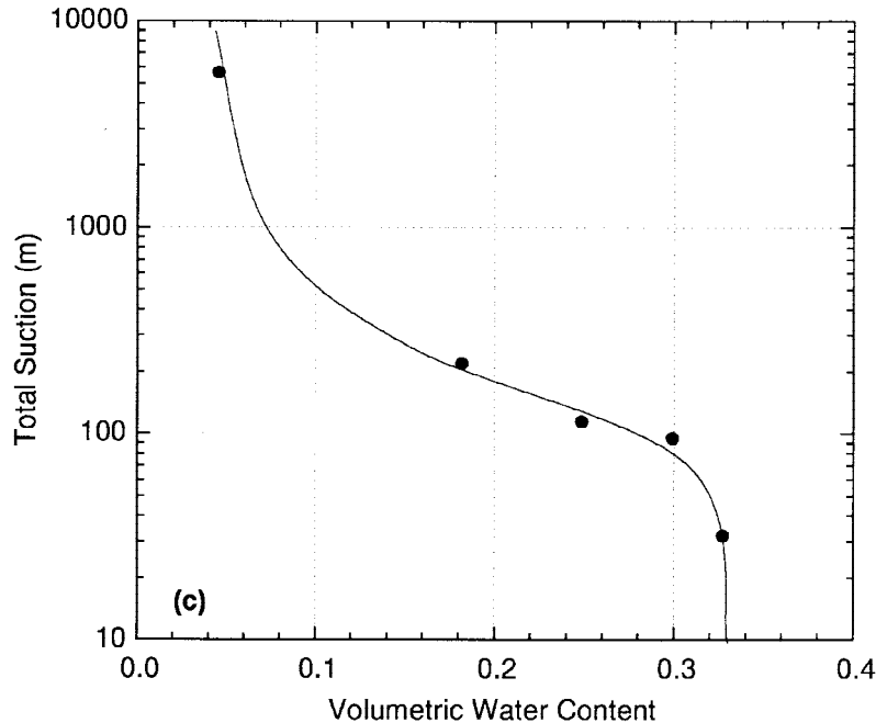
Soil water characteristic curves for (a) a clean medium sand obtained using Method A, (b) a sandy clay using a combination of Methods A, B, and D for low, moderate, and high suctions, and (c) a sandy silt obtained using Method C. All suctions reported in m of water.
