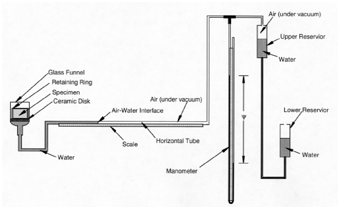
FIG. 1 Schematic of Hanging Column Apparatus
