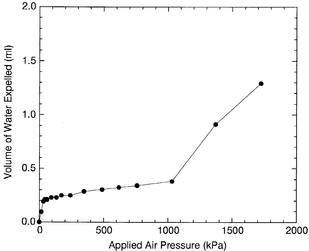
Plate function satisfactorily until a gas pressure exceeding 1000 kPa was applied, after the volume of water expelled increased dramatically. The plate was discarded. FIG. 12 Outflow from Check of a Ceramic Plate With a Reported Air Entry Pressure of 1500 kPa
