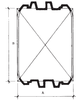
(a) Wall-Log Without Saw Kerf: Maximum allowable narrow face knot, D , determined for A \times B inscribed rectangle.
