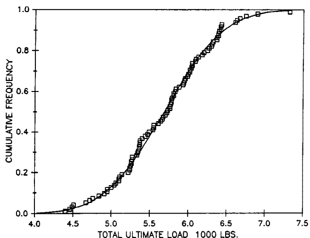
FIG. X4.1 11.875 Data and Normal Distribution
