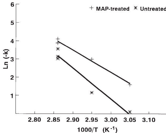
FIG. X1.2 Arrhenius Plot
