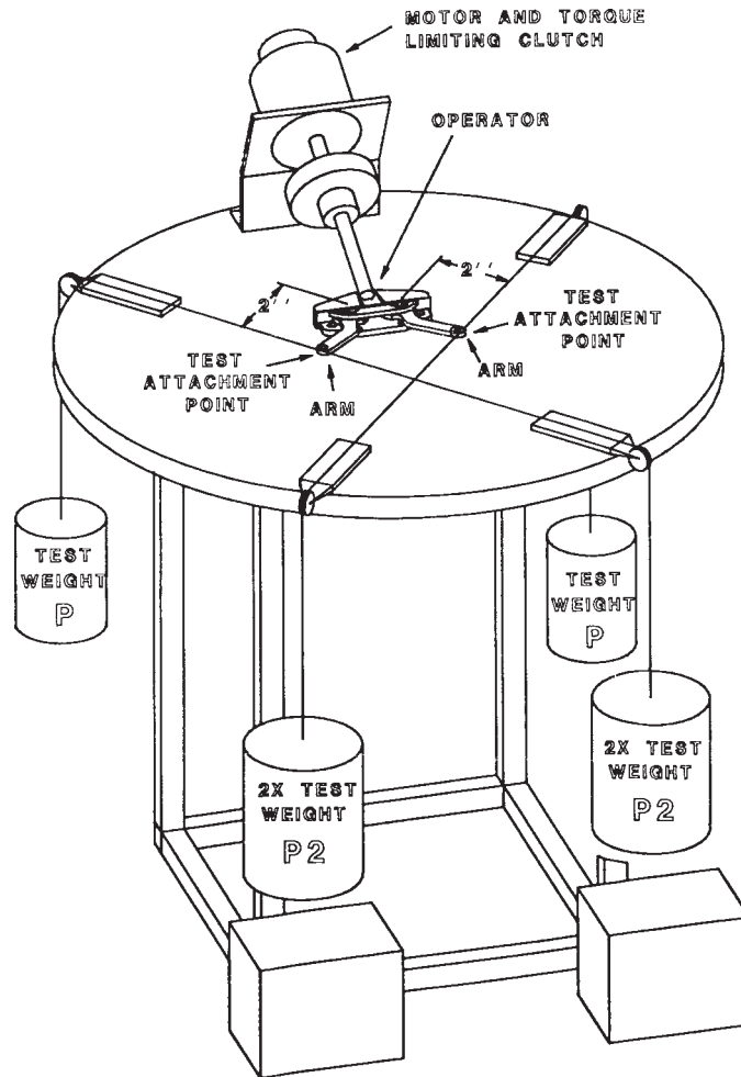
FIG. 1 Typical Operator Test Apparatus
