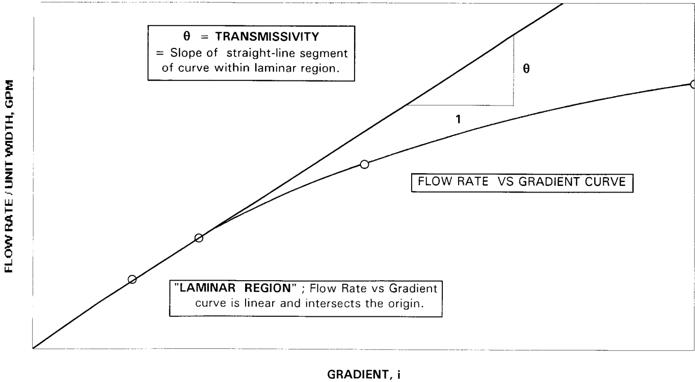
FIG. X1.1 Hydraulic Transmissivity
