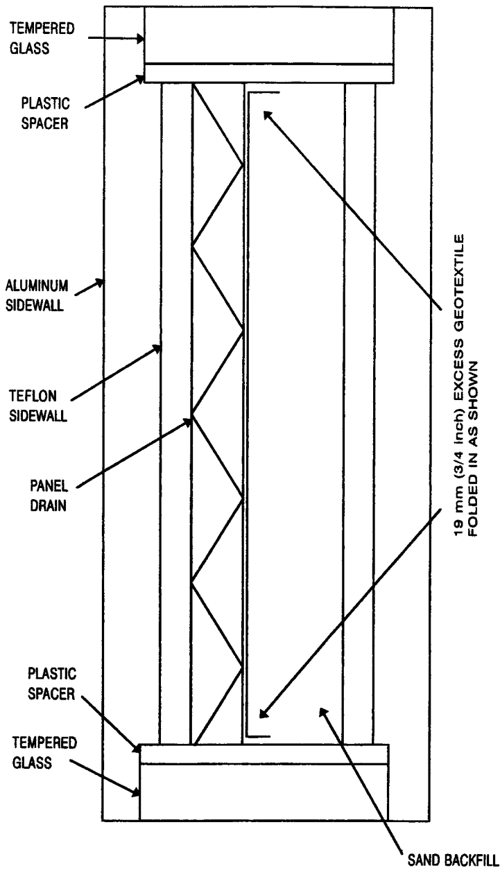
FIG. 2 Top View of Compression Chamber
