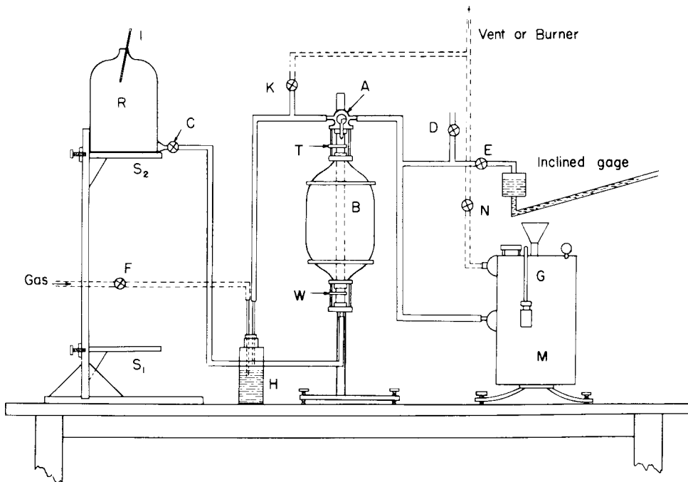
NOTE 1—Dotted lines indicate additional connections when gas is used. In this case, it may be preferable to attach the inclined gage to the meter outlet. FIG. 5 Schematic Diagram of Equipment and Connections for Calibration of a 0.1-ft 3 Wet Test Meter with a 0.1-ft 3 Bottle
