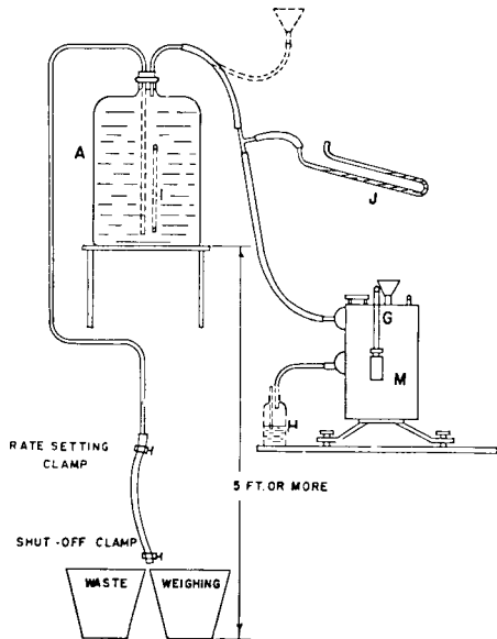
FIG. 6 Simple Equipment for Calibration by Aspirator Method
