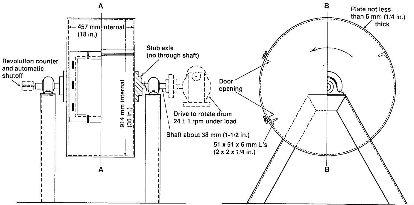
SIDE ELEVATION, HALF IN SECTION ON BB
