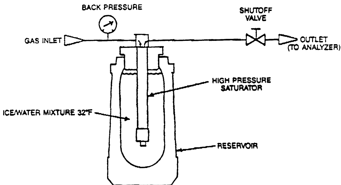
Flow Diagram
