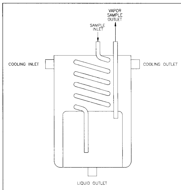
FIG. 5 Combination Condenser/Separator
