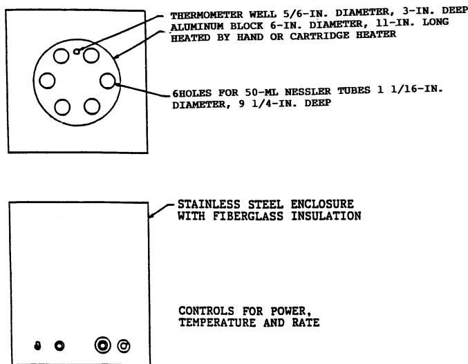
FIG. 1 Heat Stability Block
