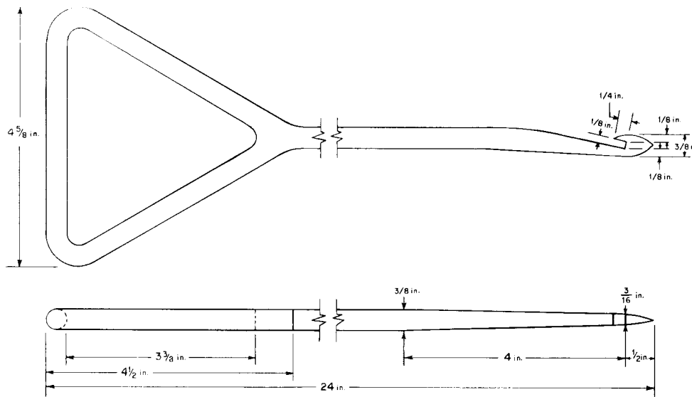
FIG. 1 Wool Staple Sampling Tool
