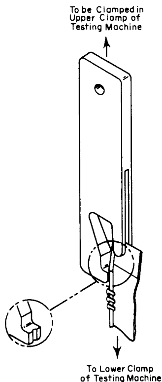
FIG. 9 Fixture for Separable Pin Pull-Off Test
