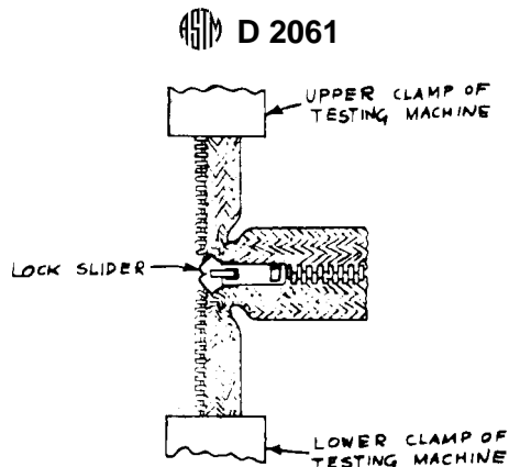
FIG. 21 Slider Lock Holding, Stringer Separation Test
