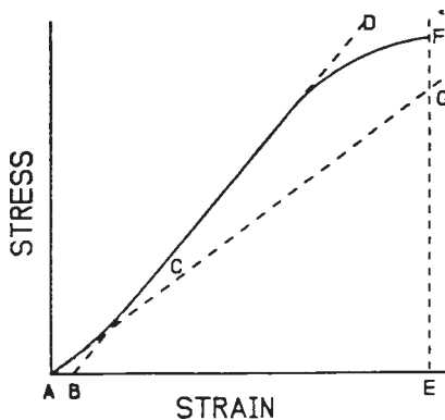
FIG. X1.1 Example of Material with Hookean Region
