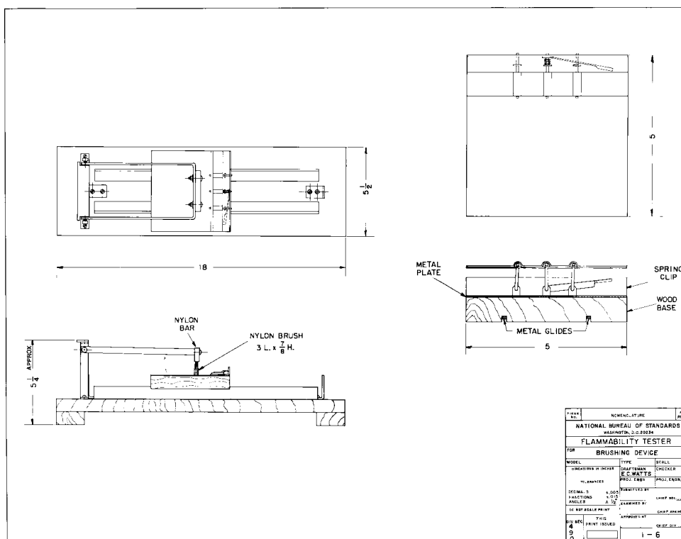
FIG. 8 Brushing Device
