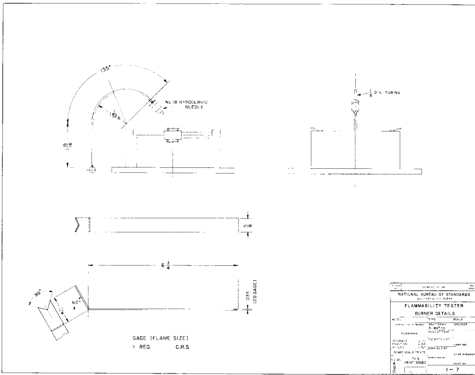
FIG. 7 Burner Details
