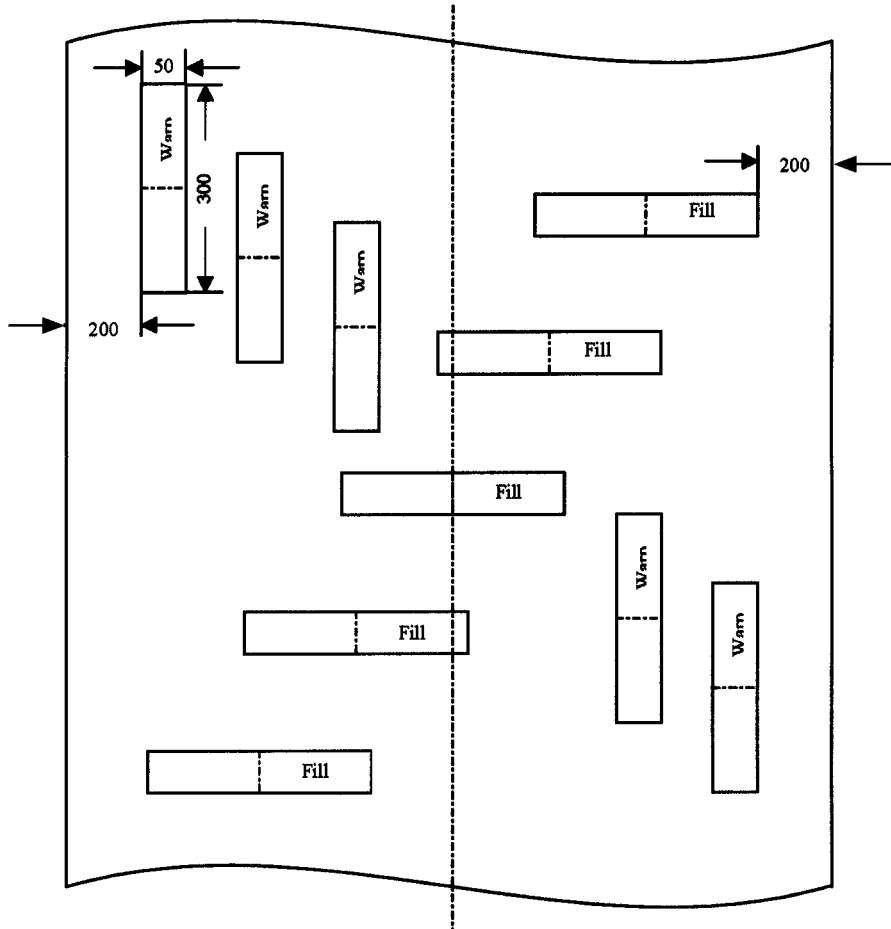
FIG. 2 Test Specimens
