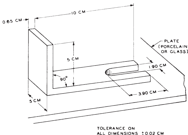
FIG. 3 Mold for Plasticizer Sorption Test
