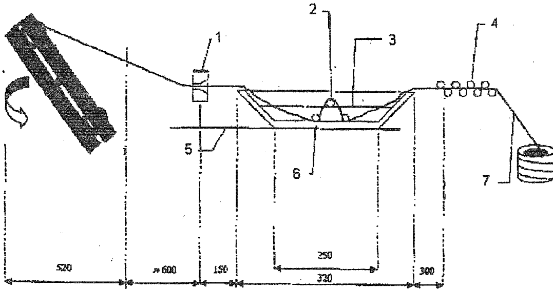
FIG. 1 Typical Impregnating Apparatus for Configurations
