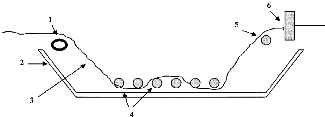
FIG. 2 Typical Impregnating Apparatus for Rovings and Yarns
