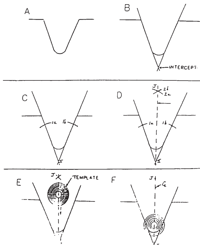
FIG. X1.4 Determination of Notching Radius
