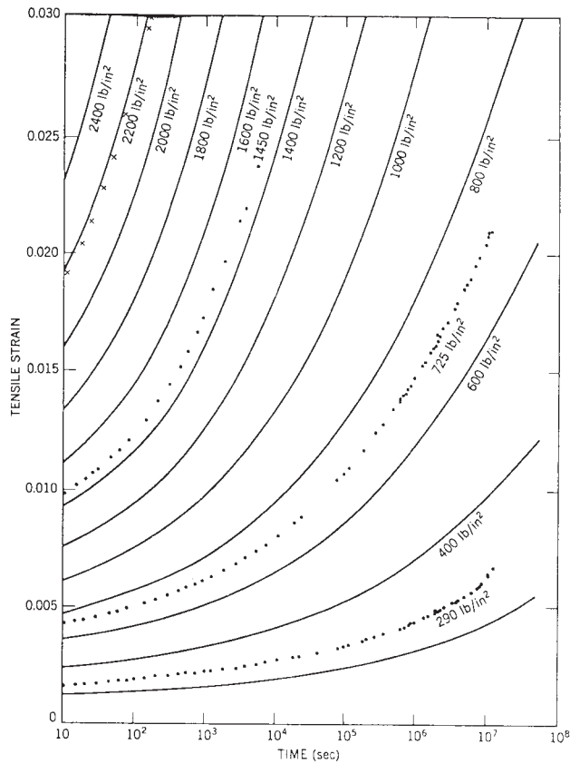
FIG. X4.2 Isochronous Data
