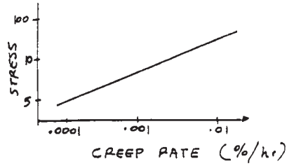
FIG. X3.2 Creep Strength
