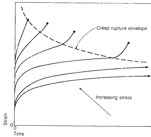
FIG. X3.4 Creep Rupture Envelope
