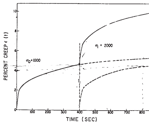
FIG. X5.1 Boltzmann Principle
