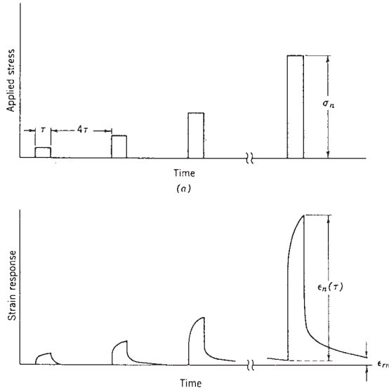
FIG. X4.2 Isochronous Data
