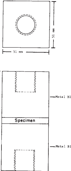
FIG. 1 Test Assembly for Bond Strength Test
