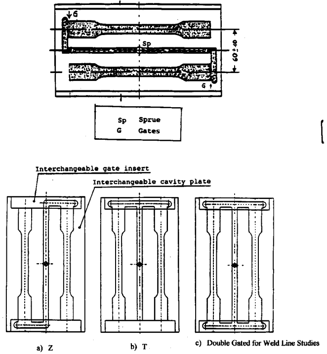
FIG. A1.2 Cavity and Runner Layout for Large Tensile Specimens
