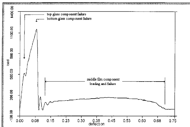
FIG. X1.5 Laminated Glass Data
