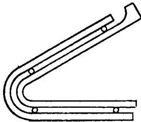
FIG. 1 Four-Point Contact System for Angular Measurement
