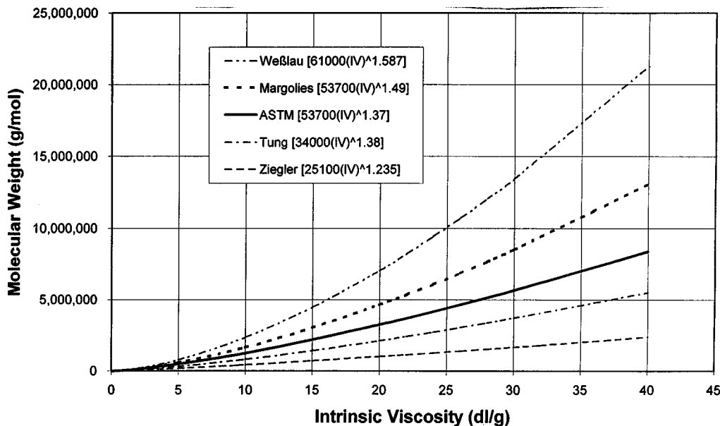
FIG. X3.1 Known Molecular Weight Equations (Correlating with Intrinsic Viscosity)
