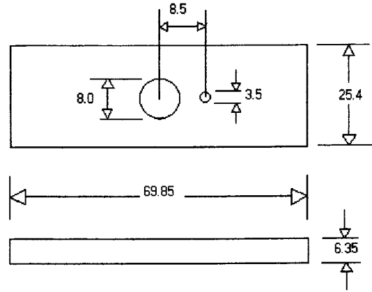
Abrasion Specimen
