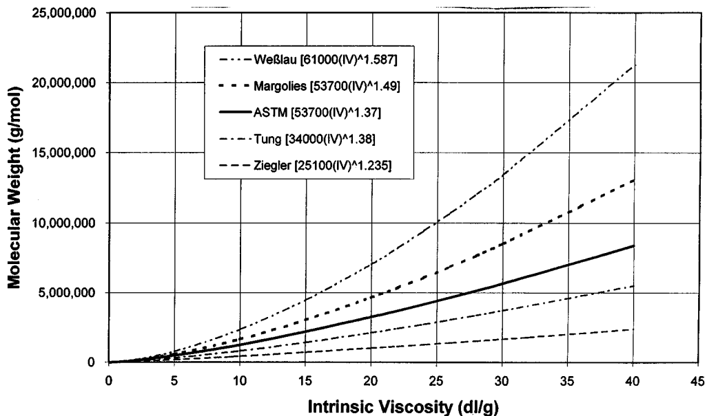
FIG. X34.1 Known Molecular Weight Equations (Correlating with Intrinsic Viscosity)
