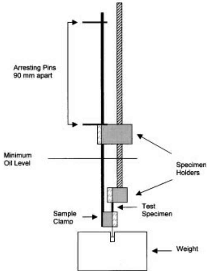
FIG. X3.2 Specimen Holder
