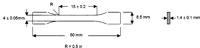
R = 0.5 in FIG. X3.1 Test Specimen
