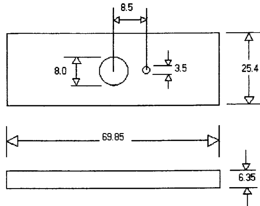
Abrasion Specimen
