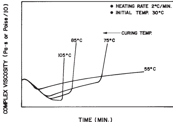
FIG. 3 Gel Point Identification of Cured Thermoset
