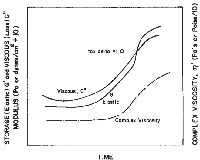
FIG. 4 Isothermal Cure Behavior After Initial Heating
