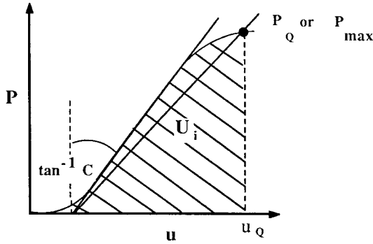
a) LOAD - DEFLECTION IN FRACTURE TEST
