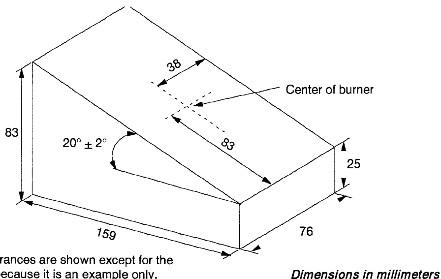
FIG. 1 Burner Mounting Block—Example
