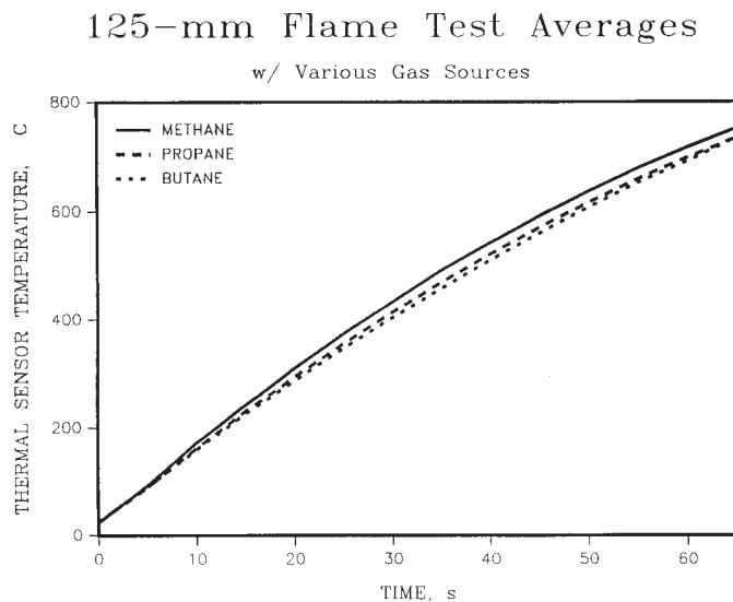
FIG. 4 Typical Temperature Response
