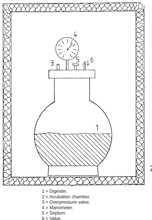
FIG. 1 Setup of Accelerated Landfill
