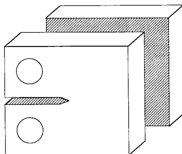
(b) Sectioning of CT Specimen.
