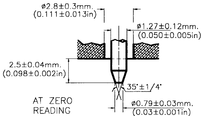
FIG. 1 (a) Type A and C Indenter
