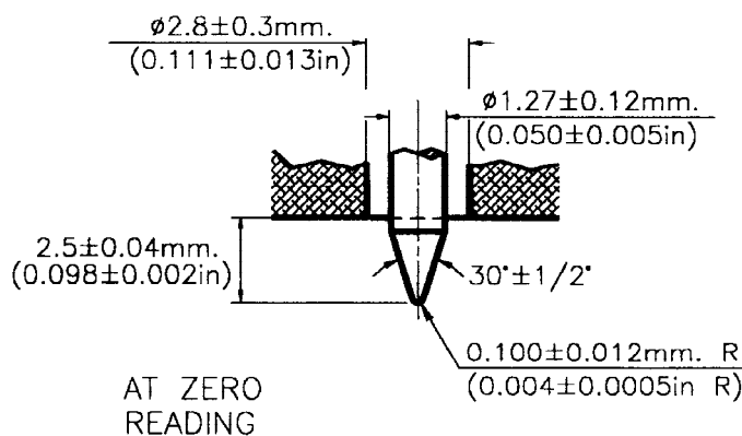
FIG. 1 (b) Type B and D Indenter (continued)
