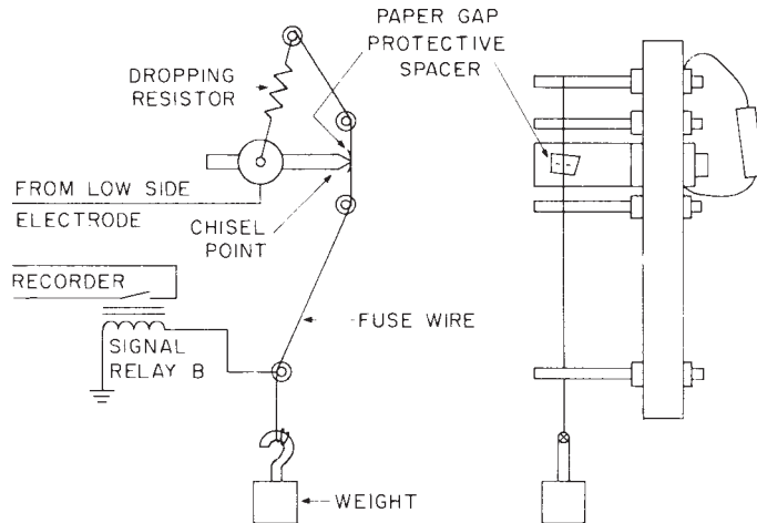
FIG. A1.12 Fusing Method of Circuit Protection
