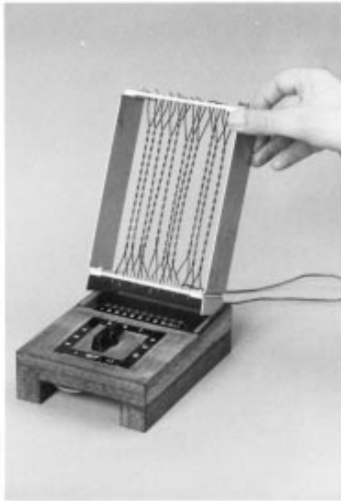
FIG. 5 Specimen Holder and Electrical Connection Device
